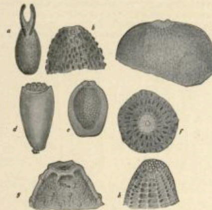
FIG. 67.—Insect eggs and parts of eggs, showing micropyle. a, egg of Drosophila celaria ; b, upper pole of egg of robber-fly, Asilus crabroformis ; c, upper pole of egg of hawk-moth, Sphinx populi ; d, egg of head-lice, Pediculus capitis ; e, egg of dragon-fly, Libellula depressa ; f, upper surface of egg of harpy-moth, Harpyia simulia ; g, upper pole of egg of Hammalicherus cerdo ; h, upper pole of egg of sulphur-butterfly, Calias hyale . (After Leuckart; much enlarged.)
